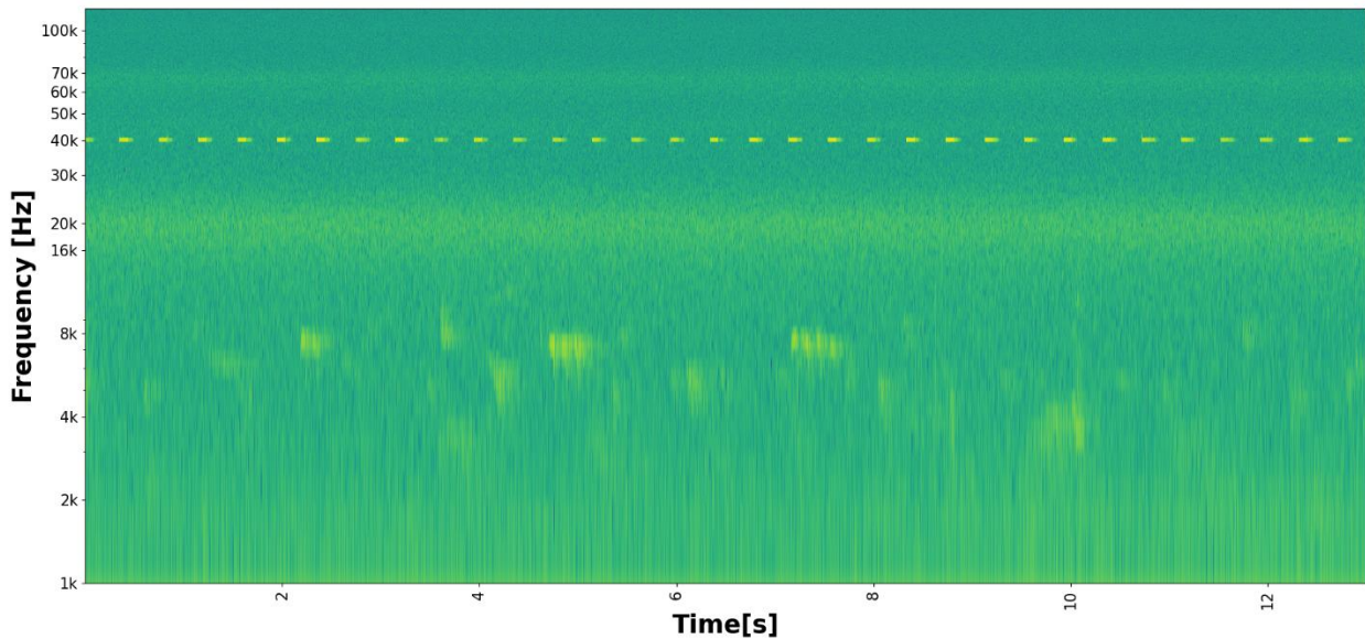
Figure 5: Spectral density plot and spectrogram for the calibration 'chirp' measured at 10 feet
