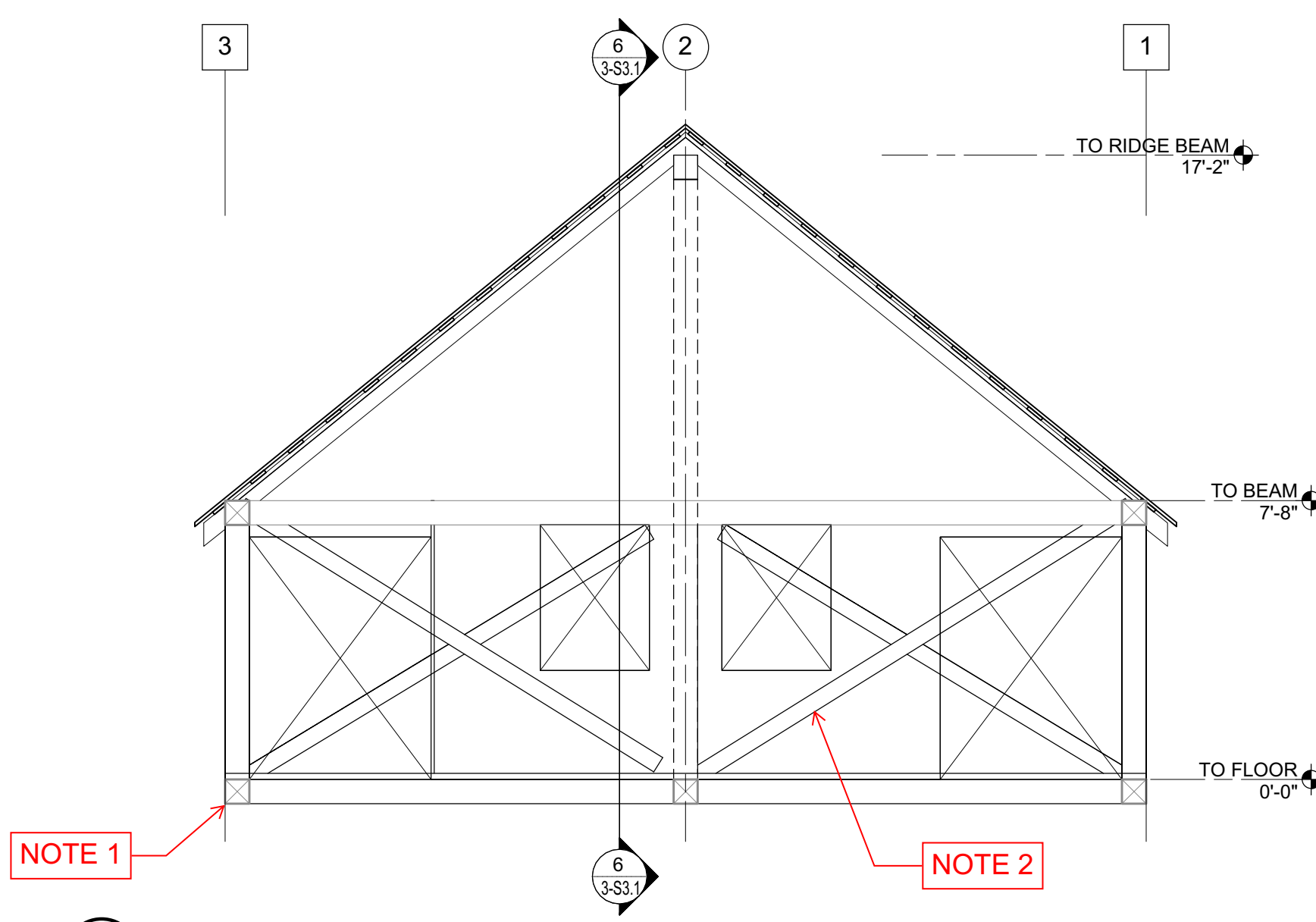
1 EAST ELEVATION BOD OPTION 2 1/4" = 1'-0"
