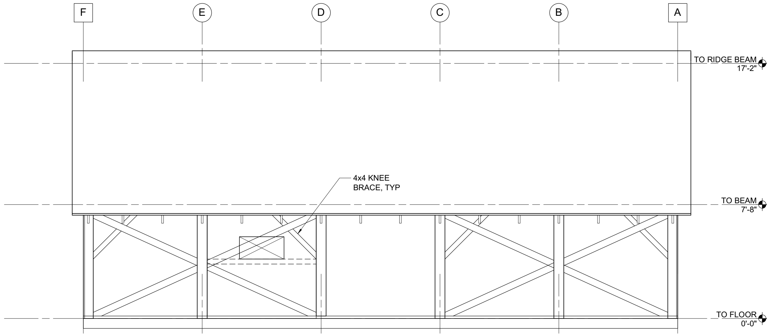
4 NORTH ELEVATION BOD OPTION 2 1/4" = 1'-0"
