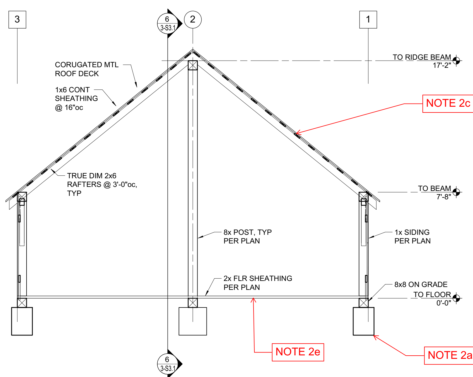
3 BUILDING SECTION - TRANSVERSE BOD OPTION 3 1/4" = 1'-0"
