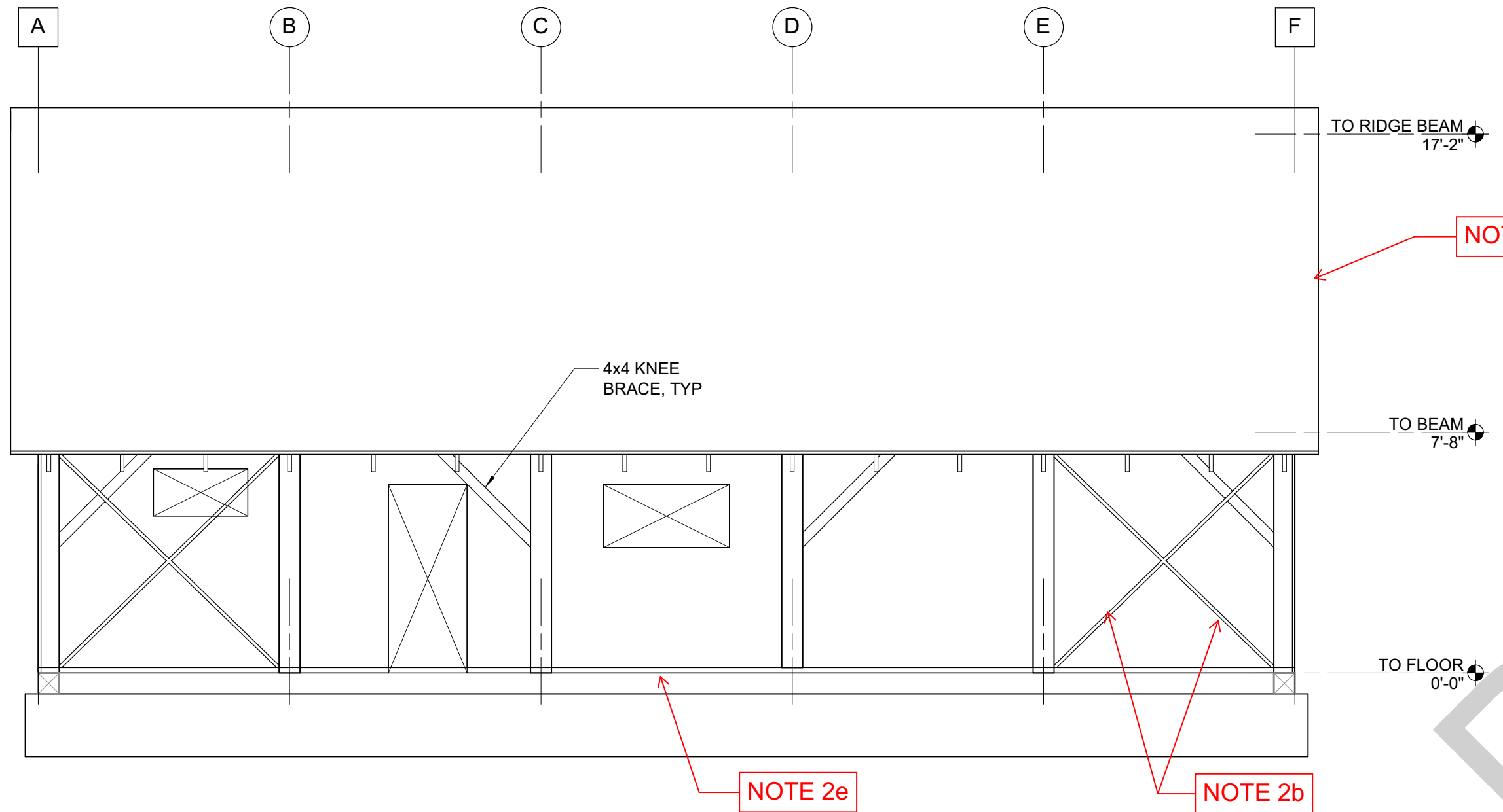
5 SOUTH ELEVATION BOD OPTION 3 1/4" = 1'-0"
