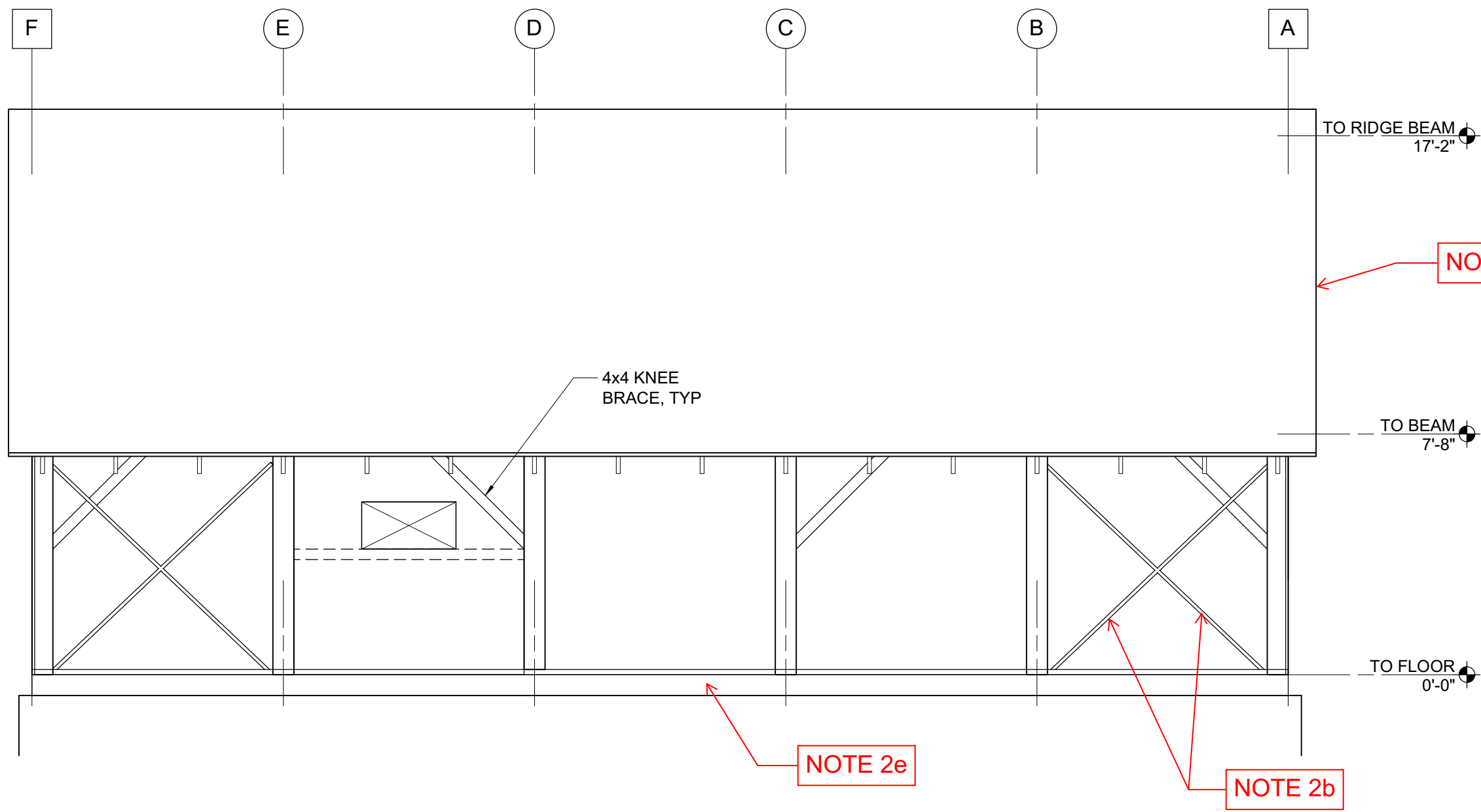
4 NORTH ELEVATION BOD OPTION 3 1/4" = 1'-0"
