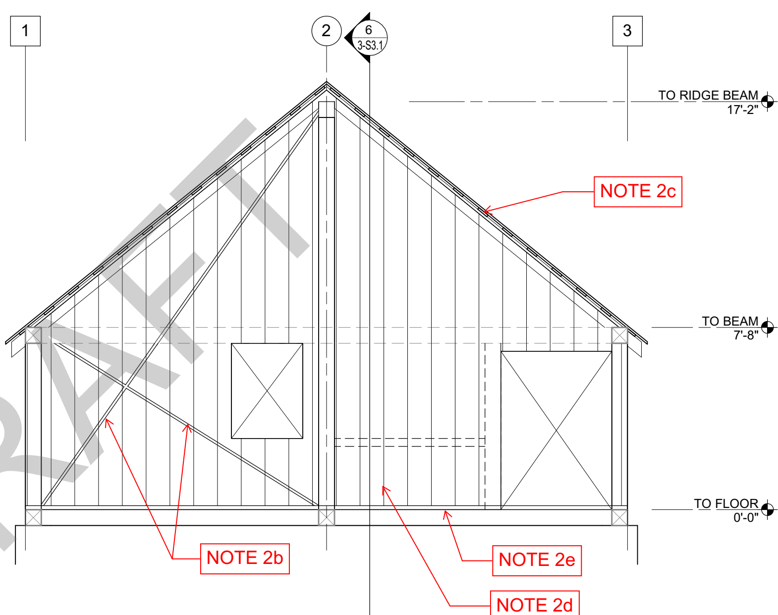
2 WEST ELEVATION BOD OPTION 3 1/4" = 1'-0"
