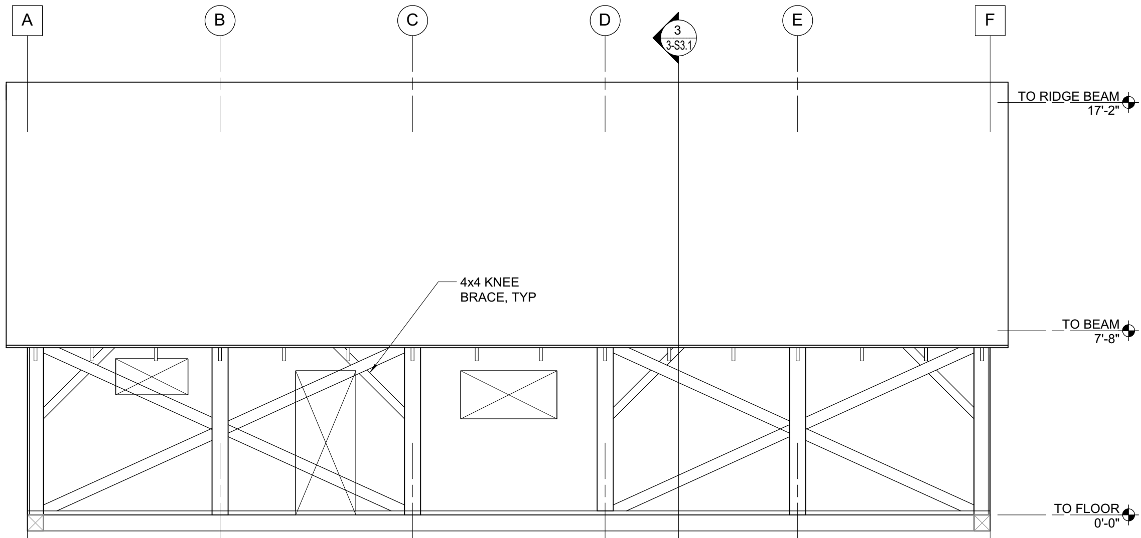
5 SOUTH ELEVATION BOD OPTION 2 1/4" = 1'-0"
