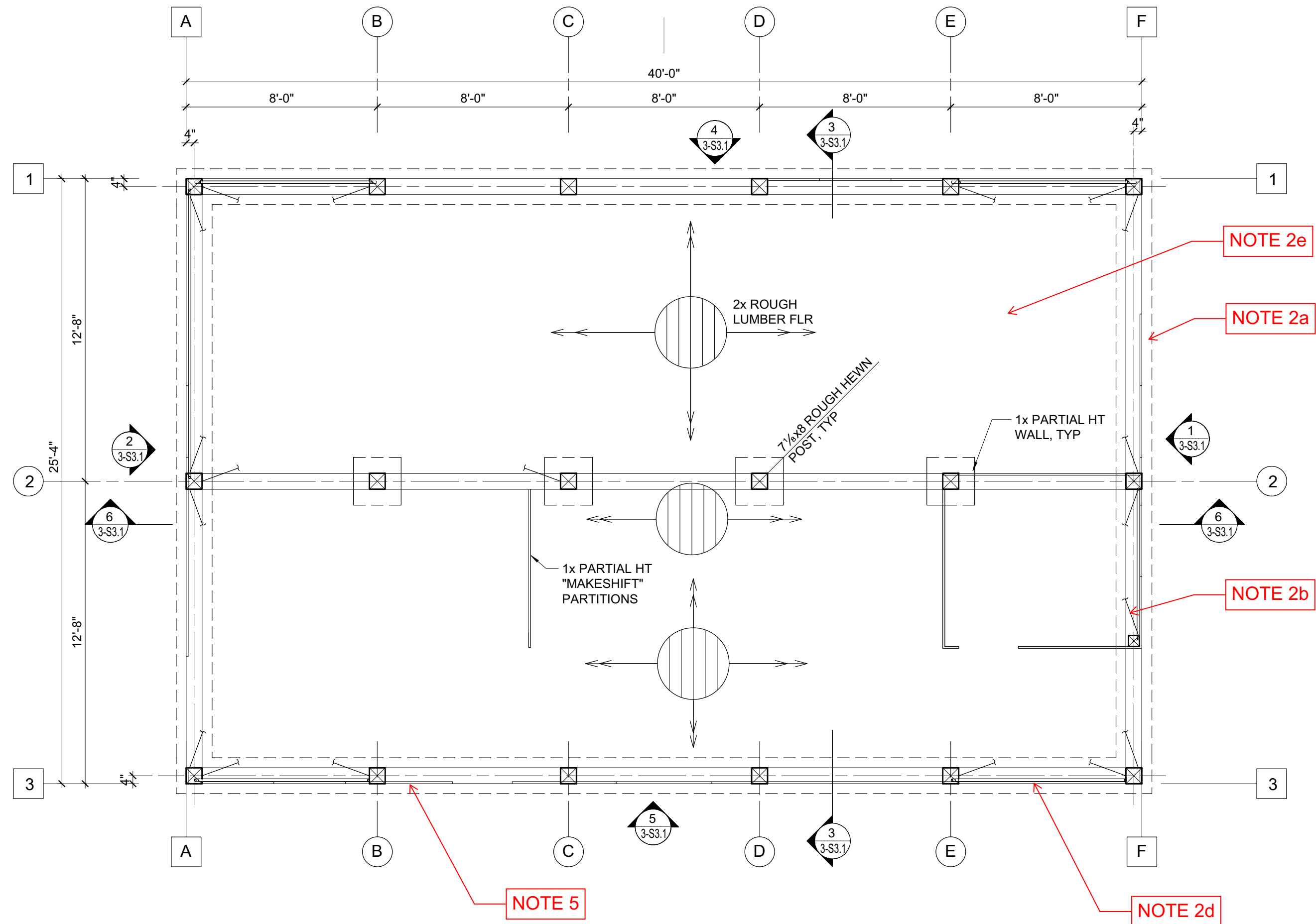
FLOOR PLAN BOD OPTION 3
