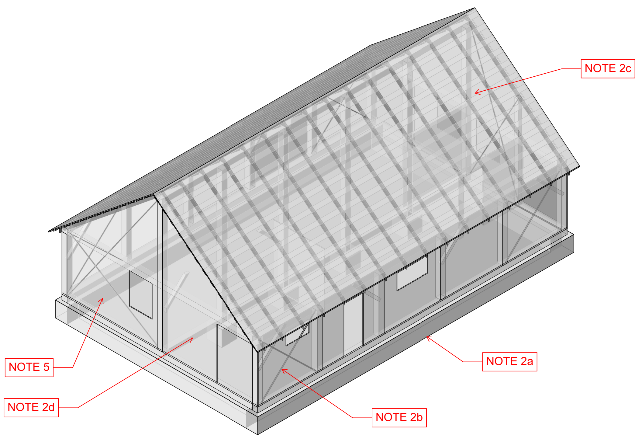
1 3D ISOMETRIC VIEW
