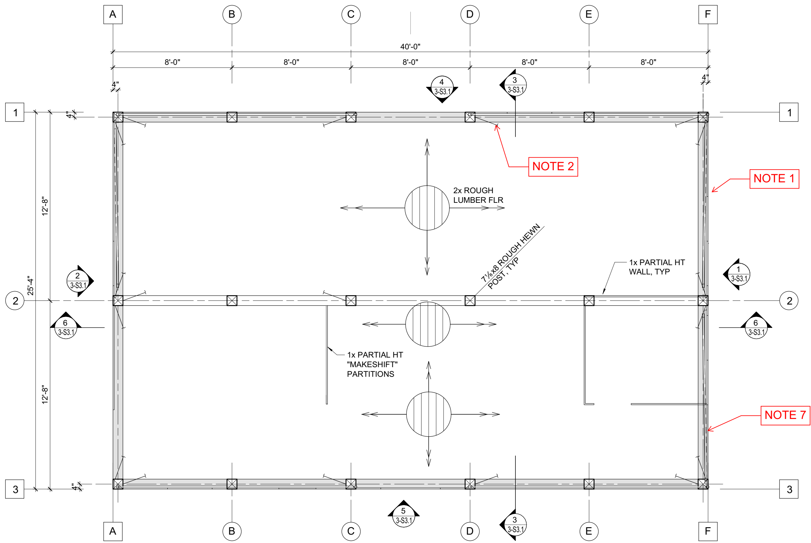
FLOOR PLAN BOD OPTION 2
