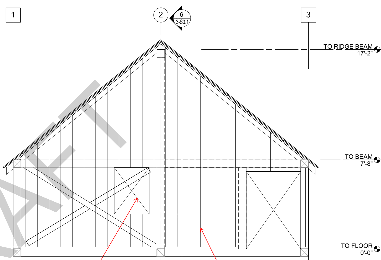
2 WEST ELEVATION BOD OPTION 2 1/4" = 1'-0"
