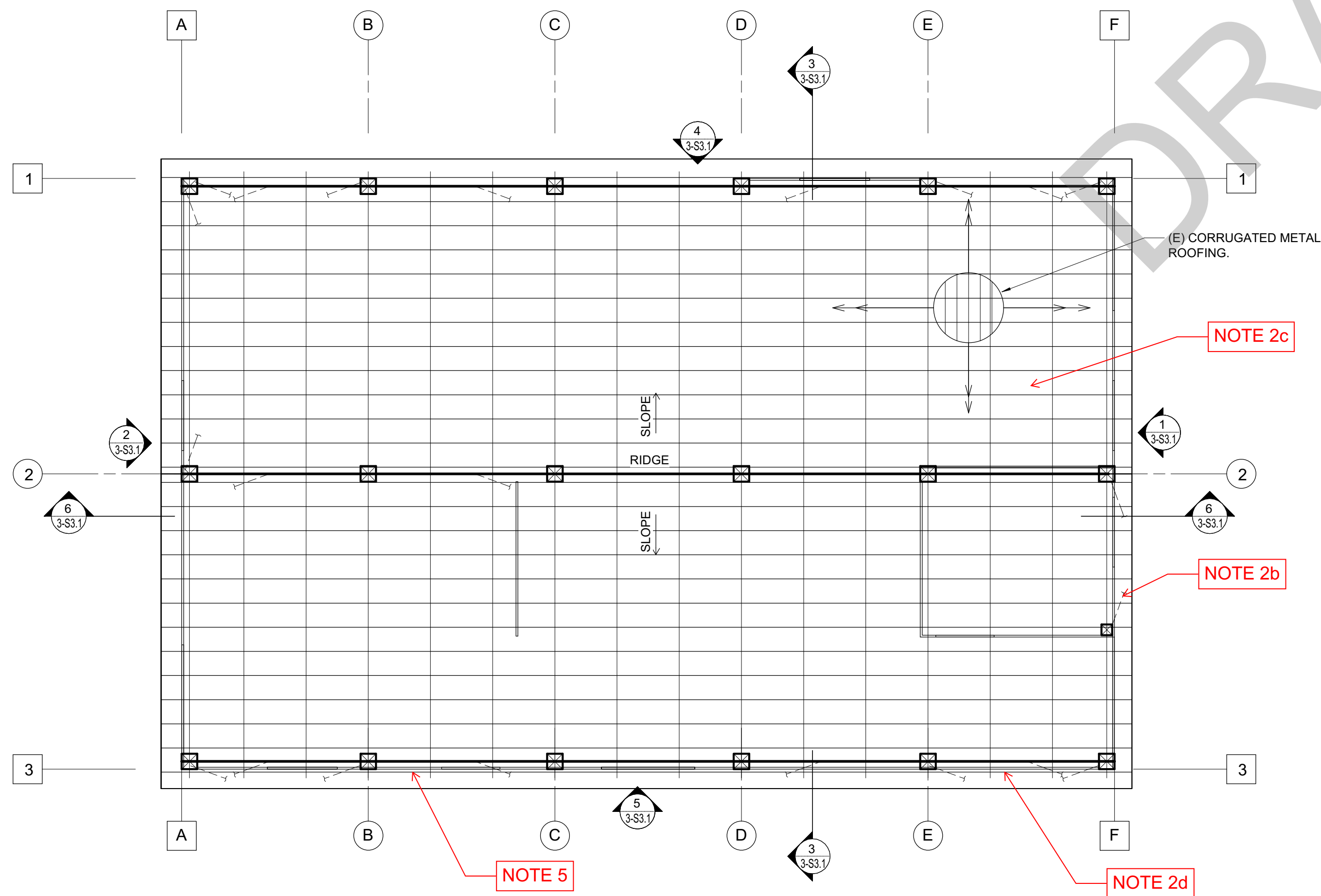
ROOF FRAMING PLAN BOD OPTION 3
