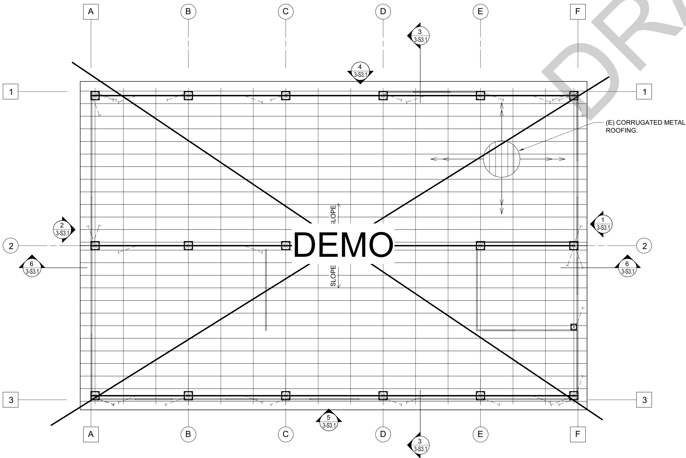
ROOF FRAMING PLAN BOD OPTION 4 1/4" = 1'-0"
