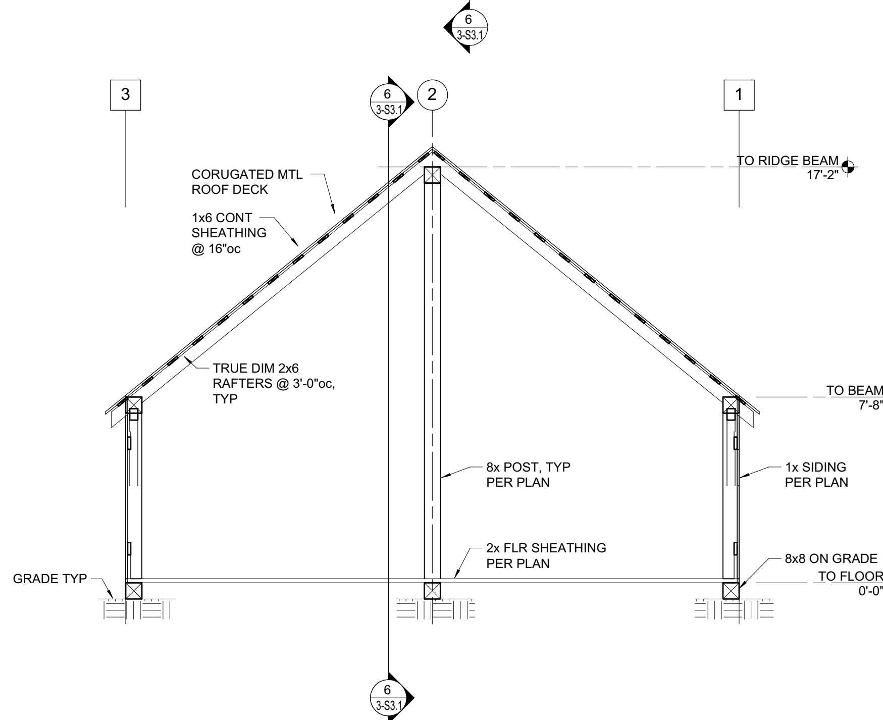
3 BUILDING SECTION - TRANSVERSE BOD OPTION 2 1/4" = 1'-0"
