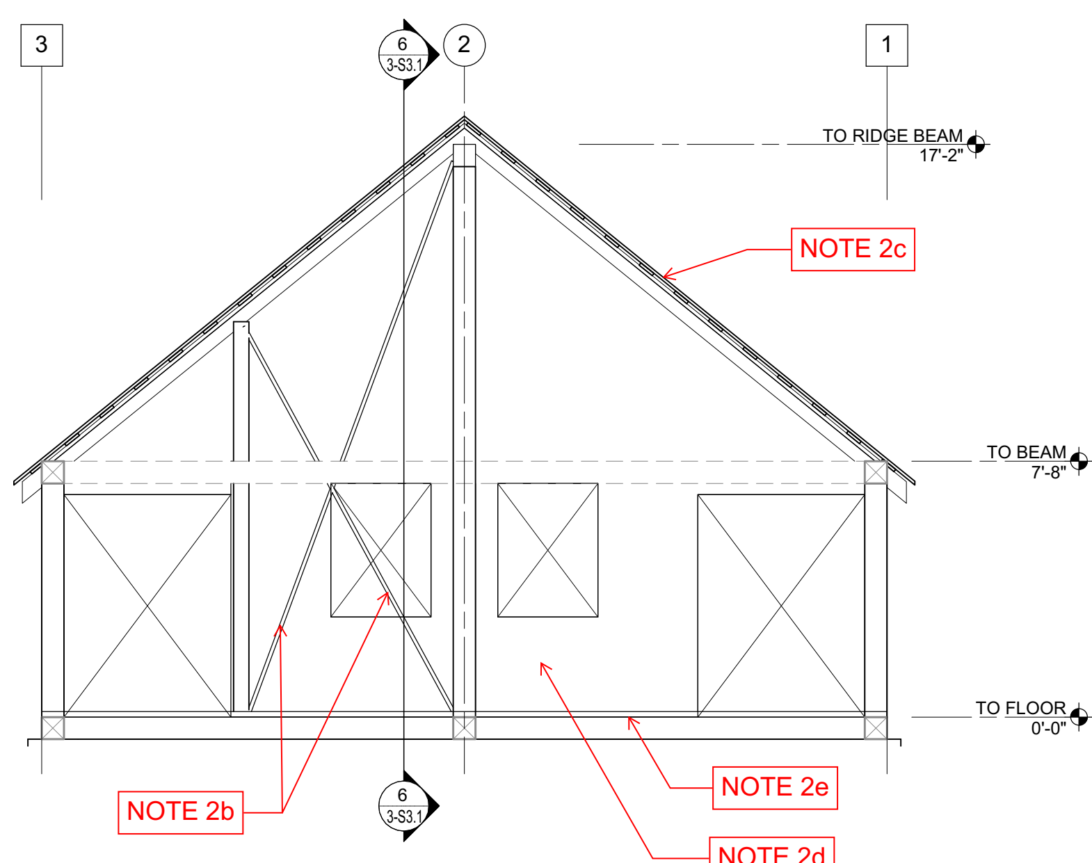
1 EAST ELEVATION C BOD OPTION 3 1/4" = 1'-0"
