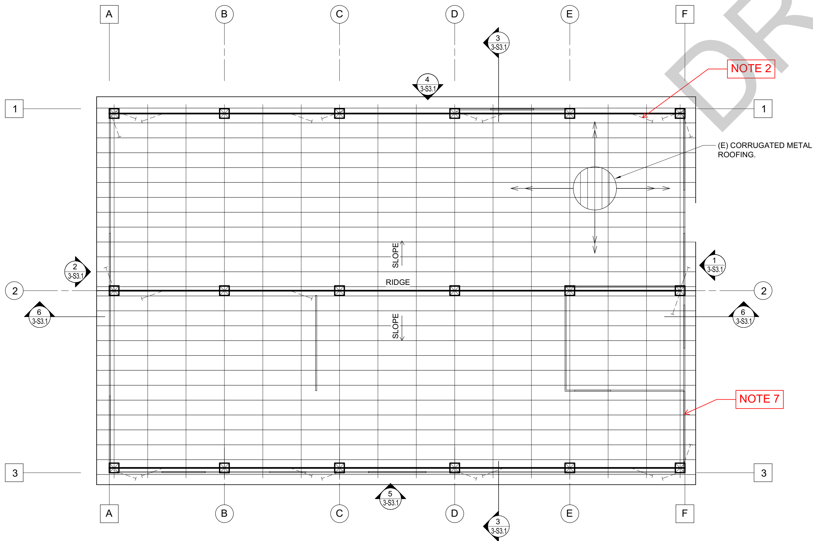
ROOF FRAMING PLAN BOD OPTION 2
