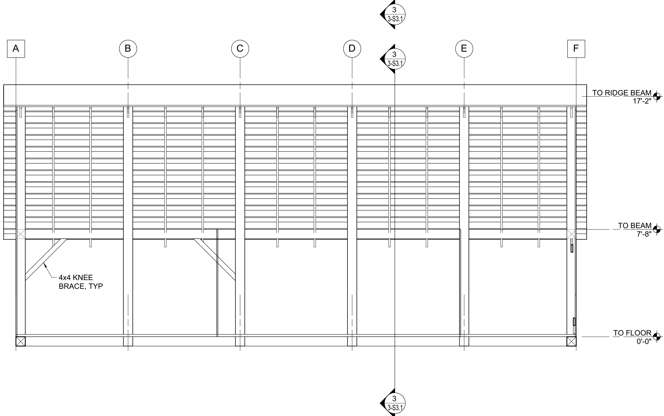
6 BUILDING SECTION - LONGITUDINAL BOD OPTION 2 1/4" = 1'-0"
