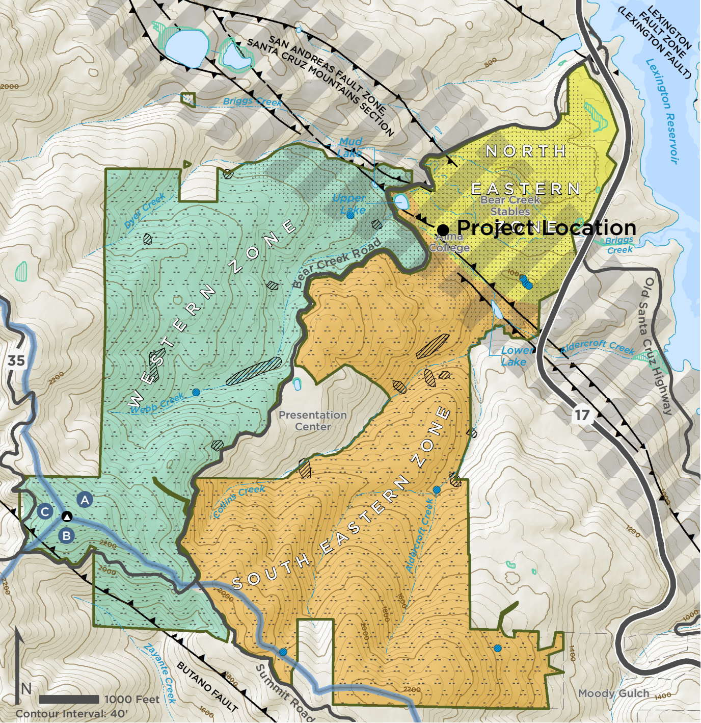
FIGURE 1 Alma College Fault Rupture Hazard Study Project Location and Geologic Base Map
